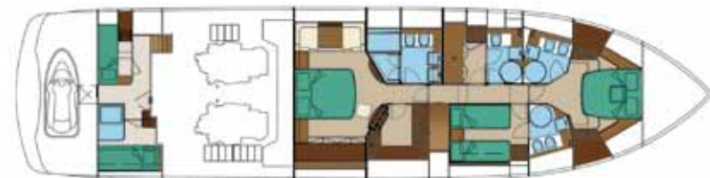
Lower deck Optional version 3 cabins + crew cabin
